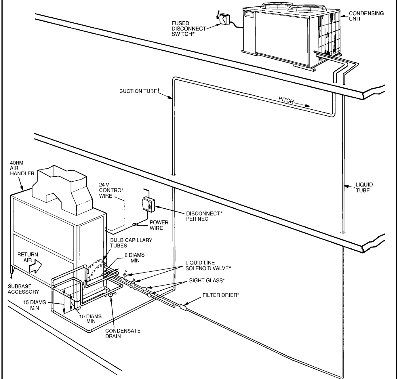
VERTICAL INSTALLATION - 40RM (TYPICAL)
